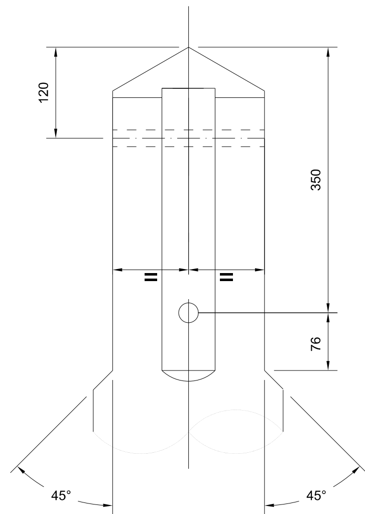
SIDE ELEVATION ON VIEW 'A' & 'B' SCALE 1:5
